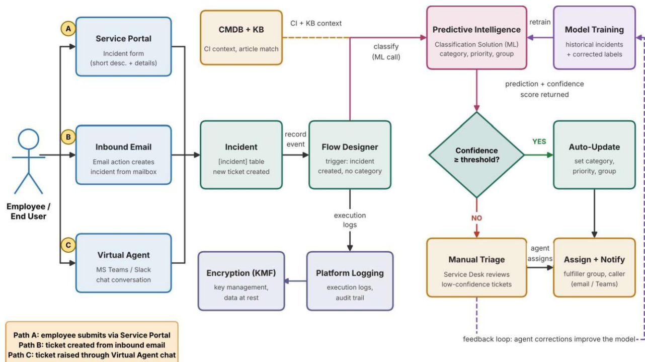
Figure 1: Architecture and data flow of the Auto Ticket Classification application
